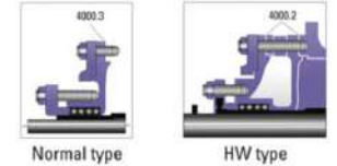
Cross section of stuffing box for MML 40, 50, 65
